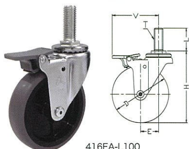
416EA-L100
